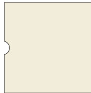
7" x 7" 1/8" Acrylic w/ 1"H x 3/8"W Thumb Cut
