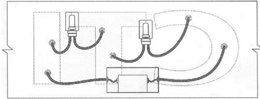
Rear view of a typical wall-mounted channel letter installation
