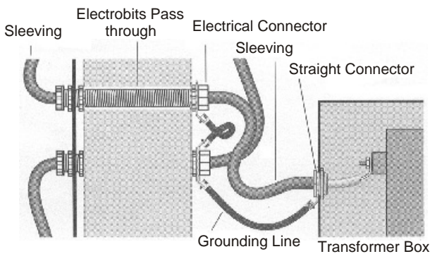
Detail showing a pass through
