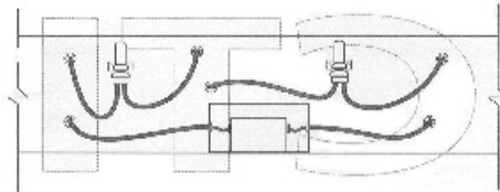
Rear view of a typical raceway-mounted channel letter installation
