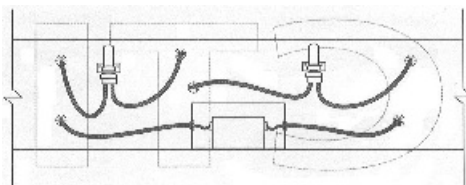
Rear view of a typical raceway-mounted channel letter installation
