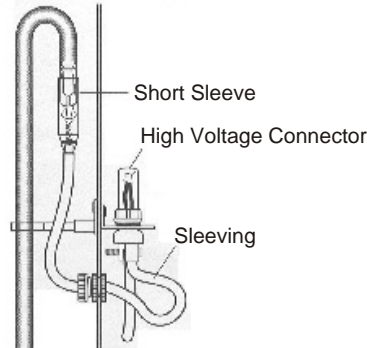
Rear view of a typical raceway-mounted channel letter installation
