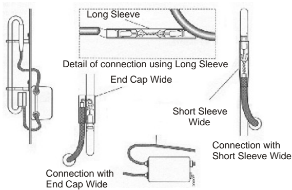
Typical installation of a window display with metal frame
