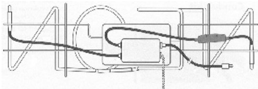
The same window display with metal frame using splice connectors, when transformer wire is too short to reach the electrode.
