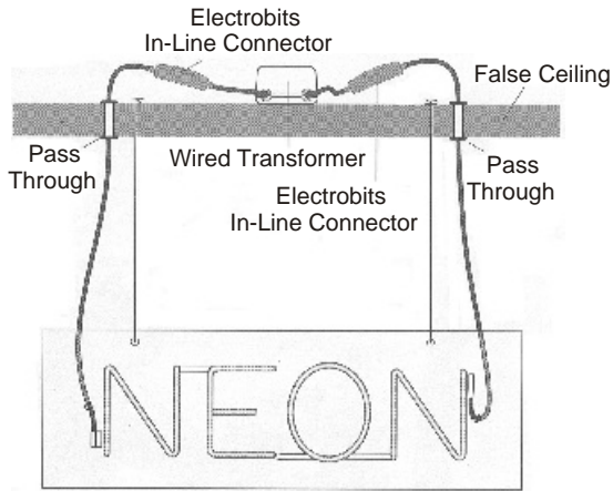
Typical installation of a window display with plastic frame
